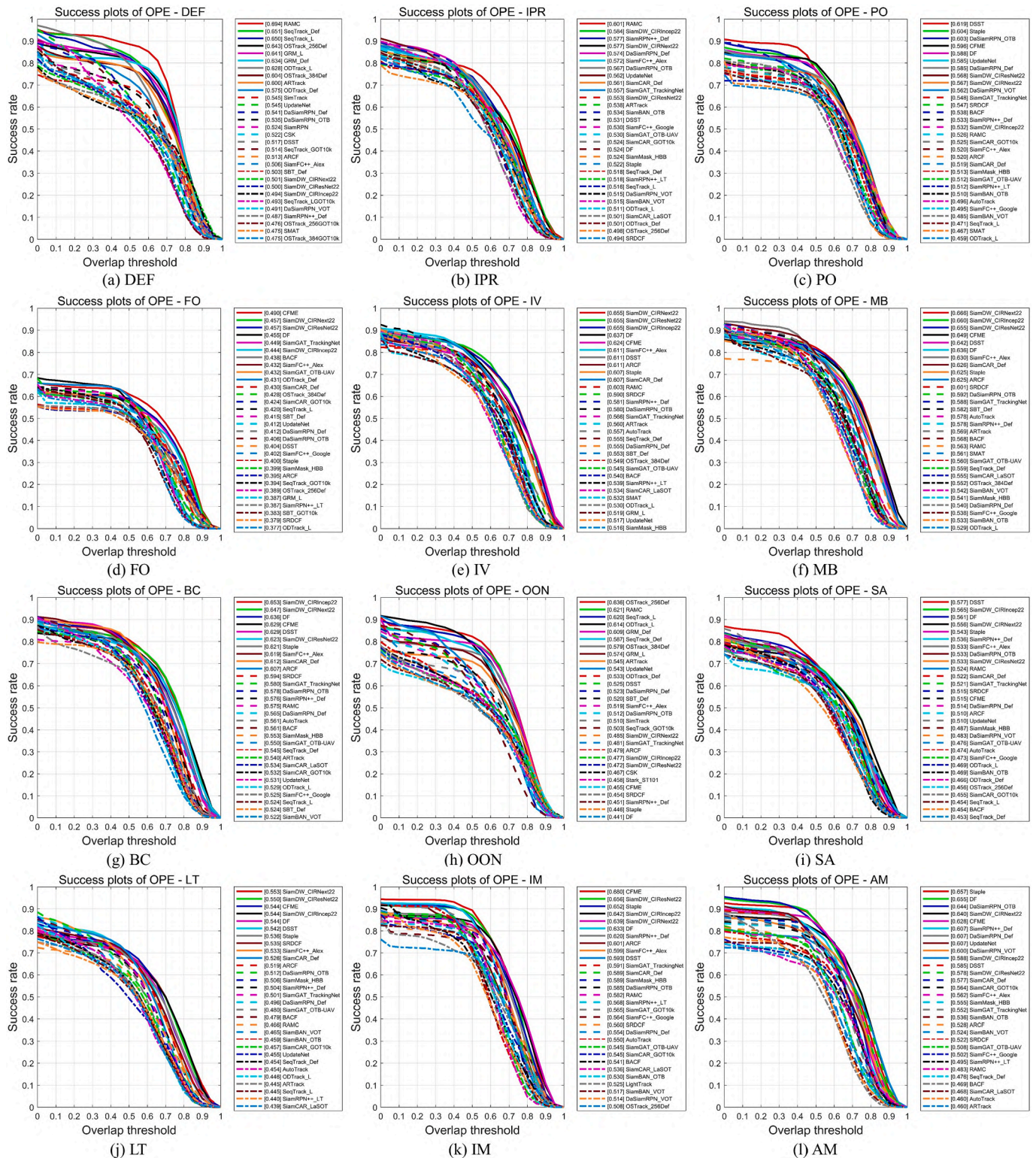
Fig. 16. The success plot of each attribute for the top 30 trackers. (a) DEF. (b) IPR. (c) PO. (d) FO. (e) IV. (f) MB. (g) BC. (h) OON. (i) SA. (j) LT. (k) IM. (l) AM.
